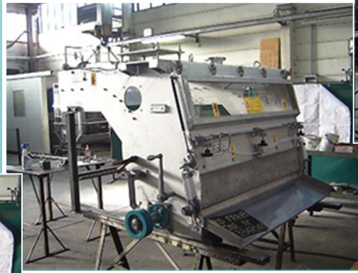
Discharge hopper pastilles/flakes with by pass
